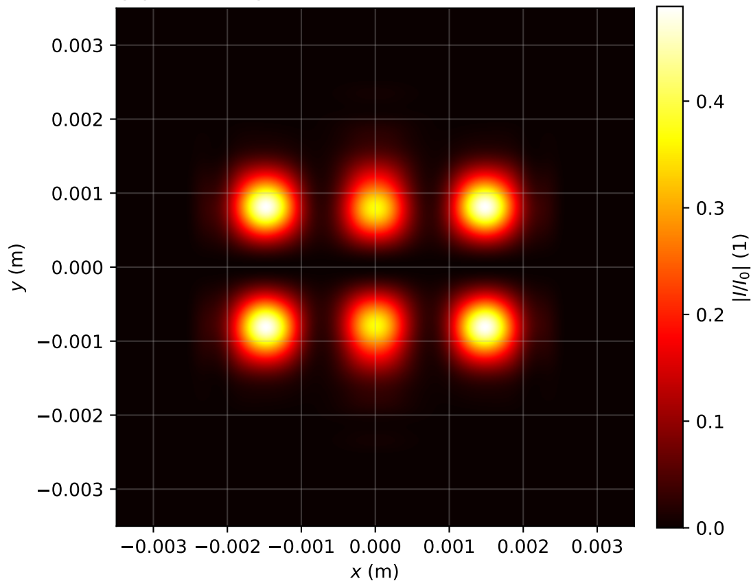
Intensity profile I(x, y, z = 3.184)/I_0 , P_{in}=3.0P_{cr} , artificial time
